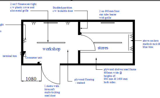
20' x 8' Workshop Stores - Plan View
