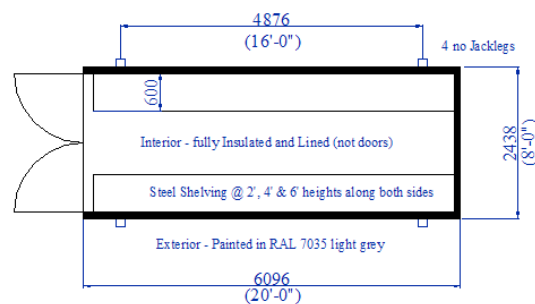
20' x 8' ISO Container Paint Stores - Plan View
